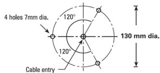
Drilling for Panel Mounting (ISO 4148)
